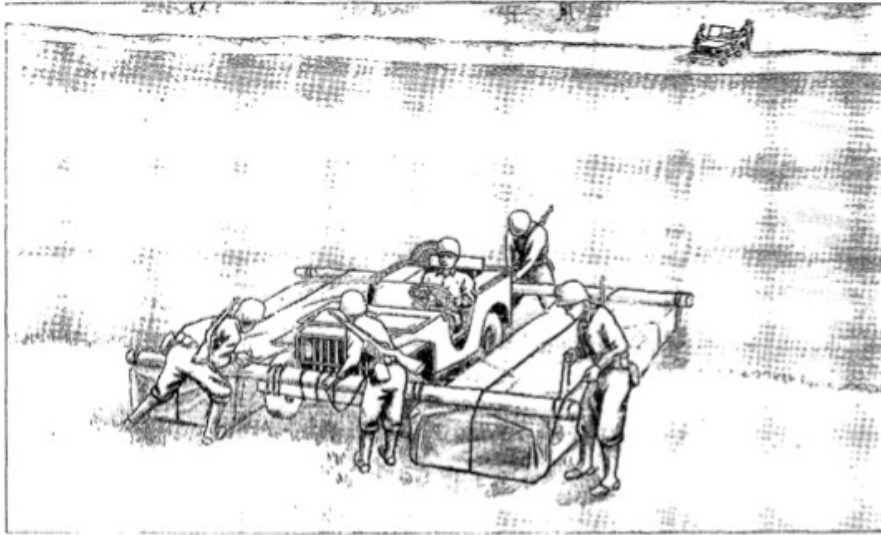
FIGURE 68.—Truck carried on outriggers. Each ponton frame should be 1½ feet by 3 feet by 11 feet.
